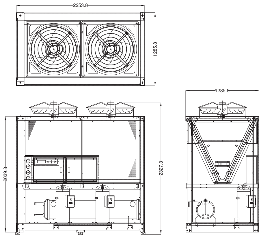
Model : 30GSU030-036
