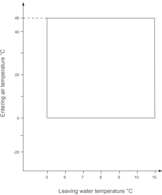
Operating range – cooling mode
