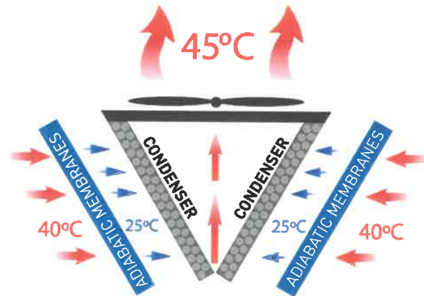
Smart Cooling adiabatic membranes
