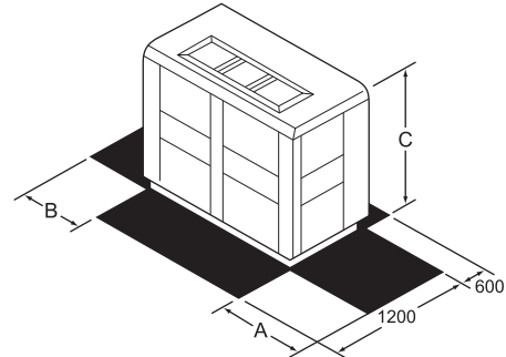
RECOMMENDED SERVICE SPACE (mm.)
