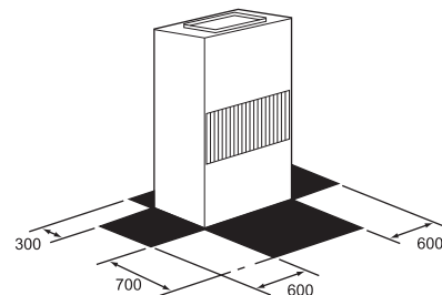
RECOMMENDED SERVICE SPACE (mm.)
