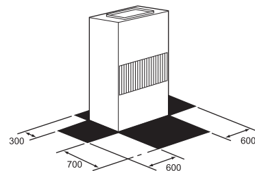
RECOMMENDED SERVICE SPACE (mm.)
